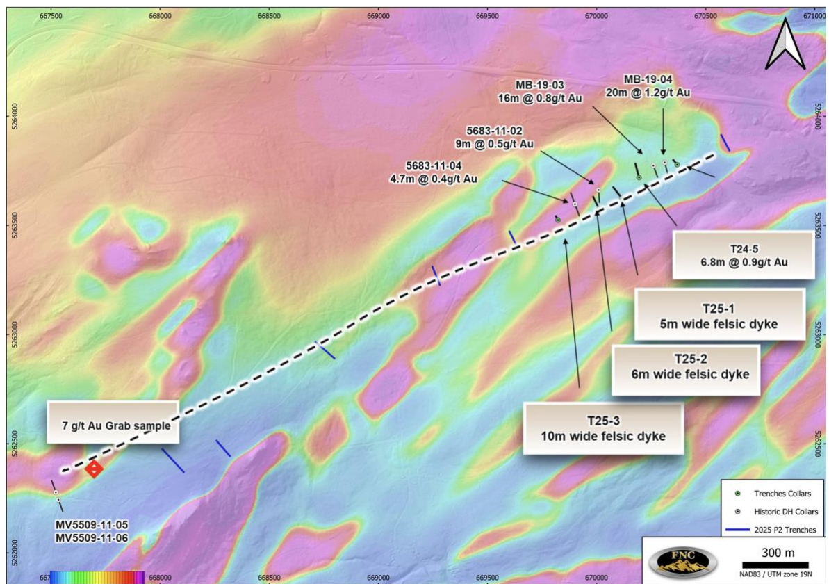
Figure 4: Area 2 McIntyre Brook Prospect with Best Assay Results and Indicating Extension of Favourable Host Horizon to a Minimum Strike Length of 3 km
