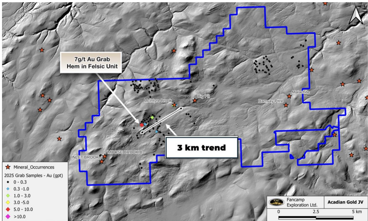
Figure 3: Acadian Gold McIntyre Brook Prospect featuring 3 km Long Trend
