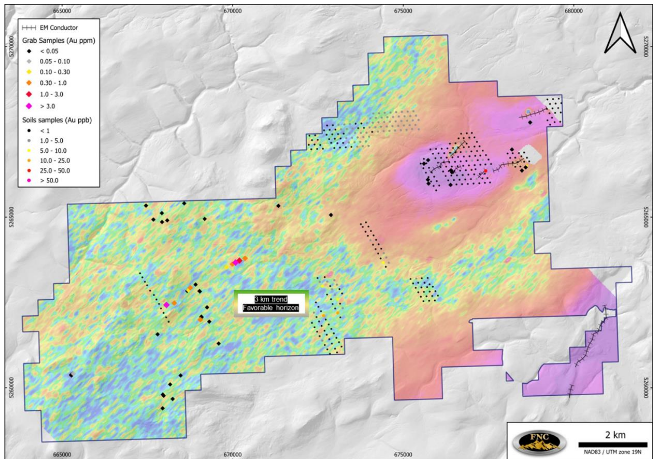
Figure 2: McIntyre Brook 2025 Soil Geochemical Superimposed on Airborne Magnetometer (1VD) Survey
