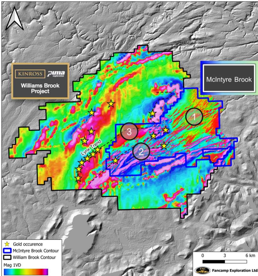
Figure 1: McIntyre Brook Prospects – (1) EM Zone, (2) McIntyre Brook Prospect and (3) Northwest Area
